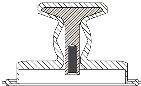
SECTION VIEW
